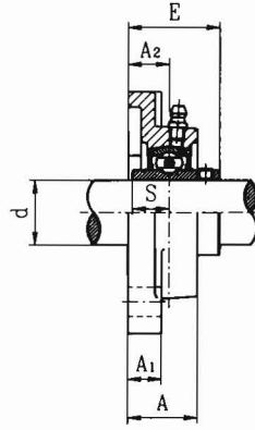
UCF2 Setscrew type
